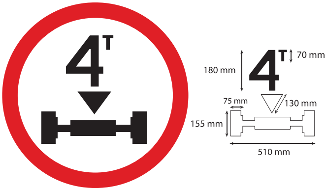
Fig 14.34 Axle Load Limit
