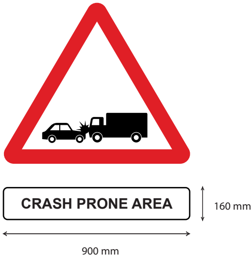
Fig 15.72 Crash Prone Area Ahead
