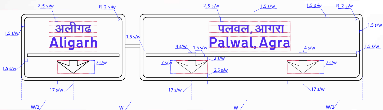
Fig. 16.13 Lane Dedicated Gantry Signs
