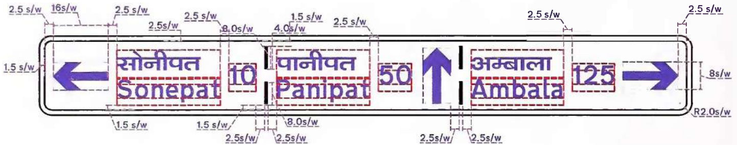
Fig. 16.11 Gantry Mounted Advance Direction Ahead of a At-Grade Junction
