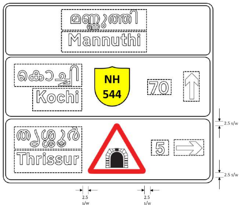
Fig. 16.01a Inclusion of Regulatory and Cautionary Signs in Advanced Direction Sign
