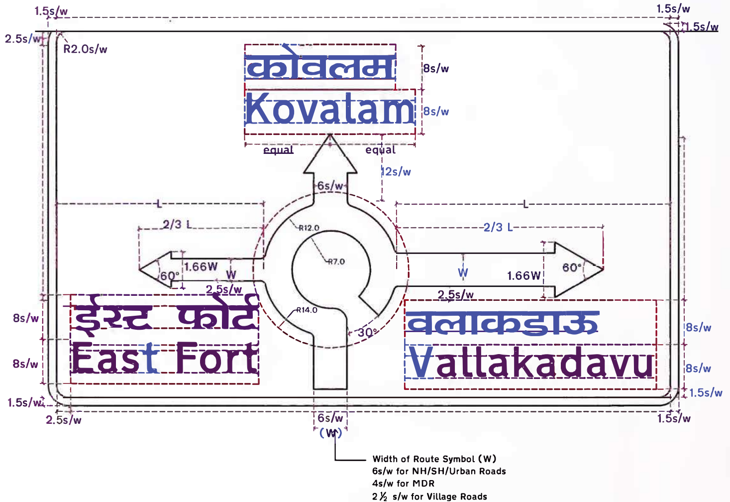
Fig. 16.03 Map type Advance Direction Sign on Roundabout (Shoulder Mounted)
