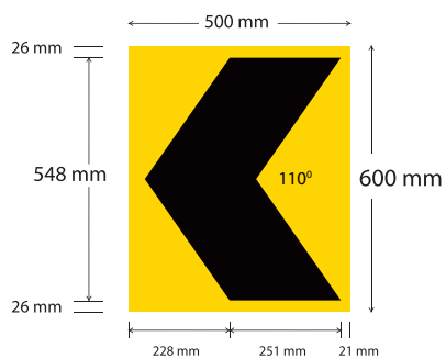
Fig 15.74 Single Chevron (Normal)
