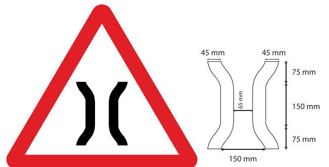
Fig 15.25 Narrow Bridge Ahead
