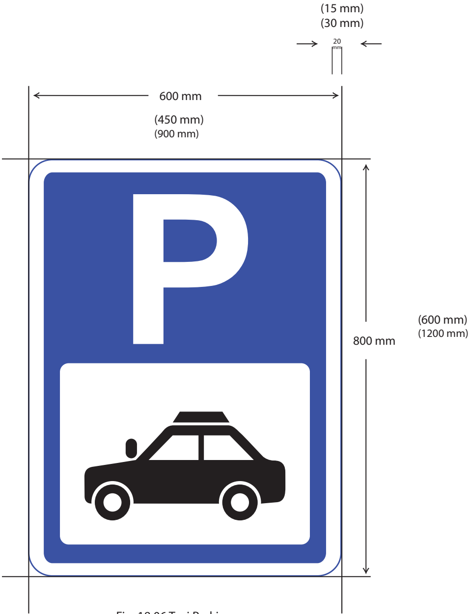
Fig. 18.06 Taxi Parking
