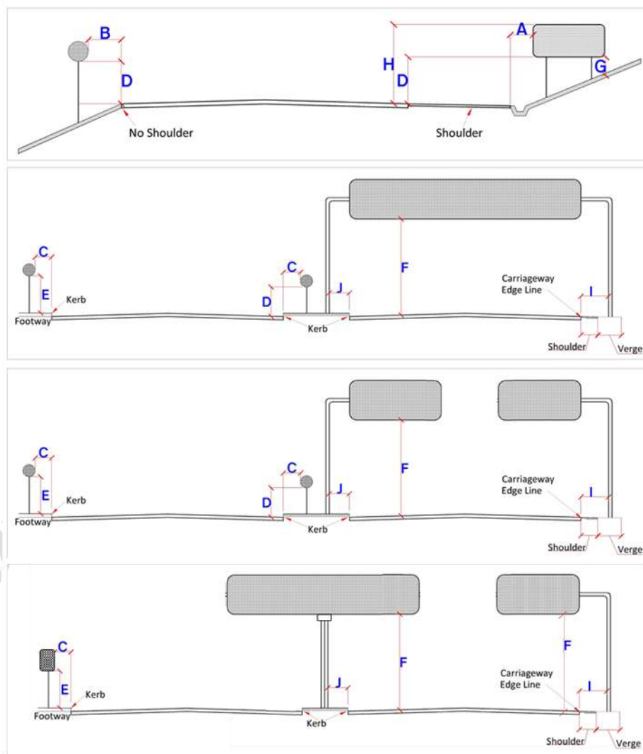
Figure 4.1: Typical Siting of Signs with respect to Carriageway (Heights and Clearances) (Refer Table 4.1 for values)
