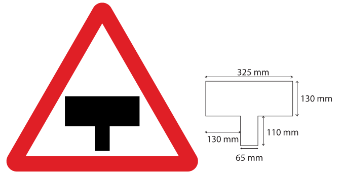
Fig 15.18 T- Intersection Major Road Ahead
