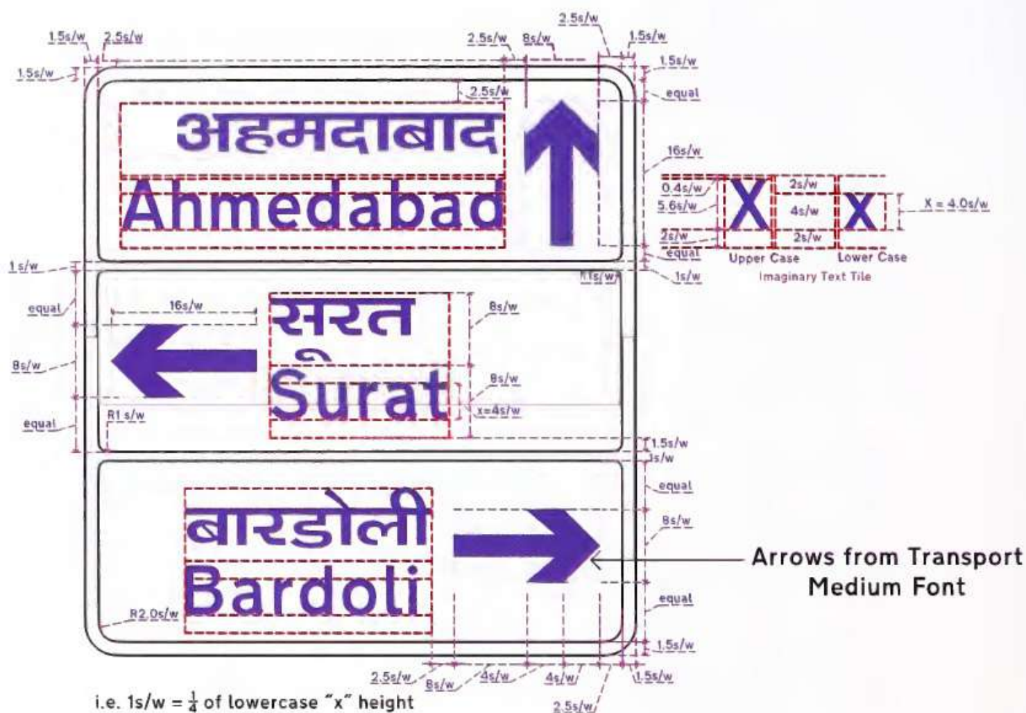
Fig. 16.01 Stack type Advance Direction Sign (Shoulder Mounted)
