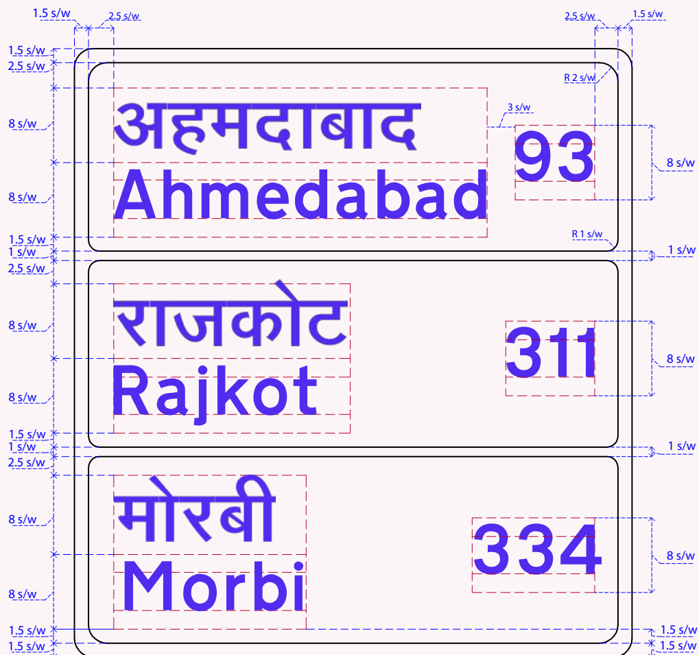
Fig. 16.04 Flag Type Direction Sign
