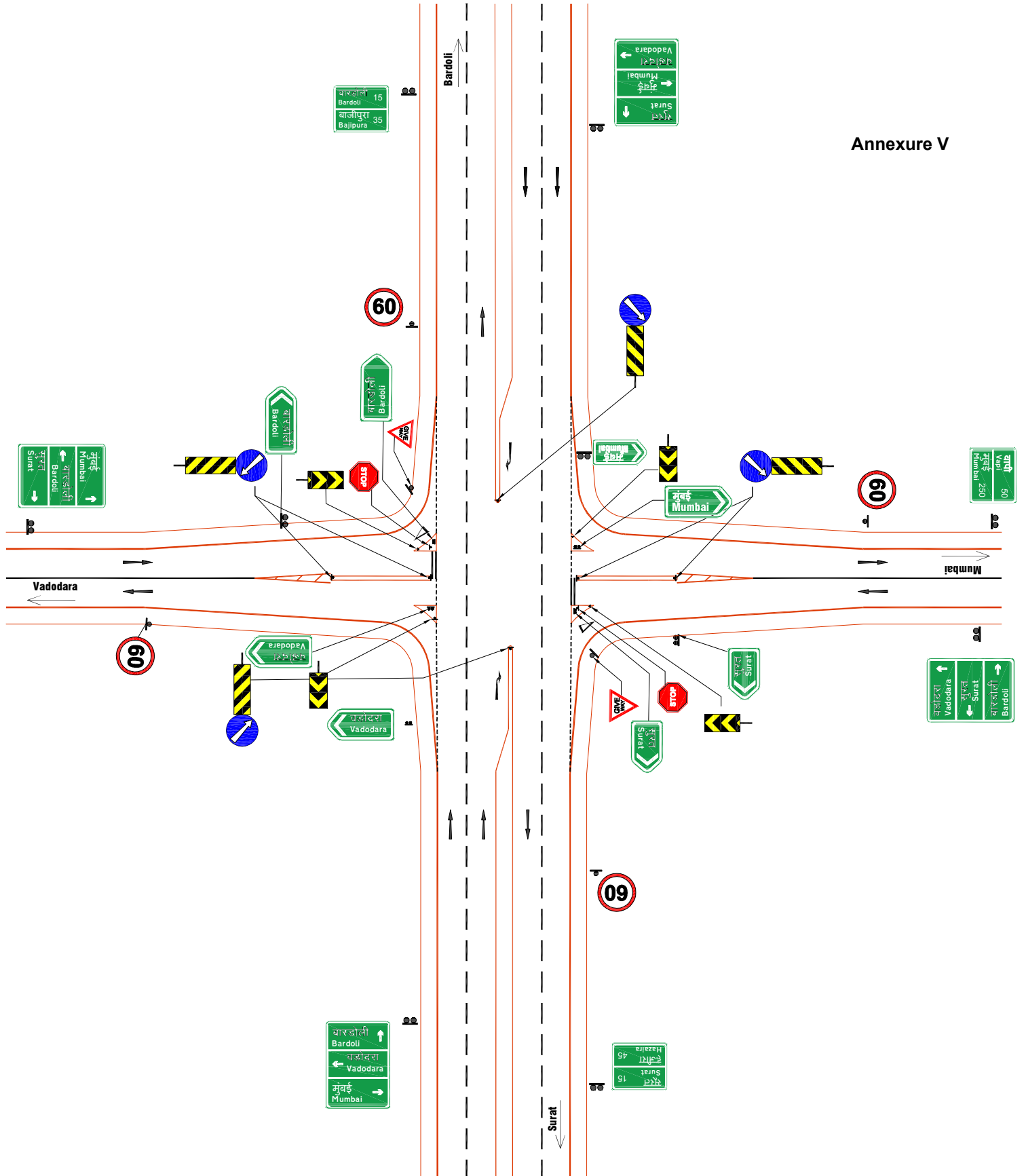
Fig V.2 Sign Plan for 4 arm priority Junction
