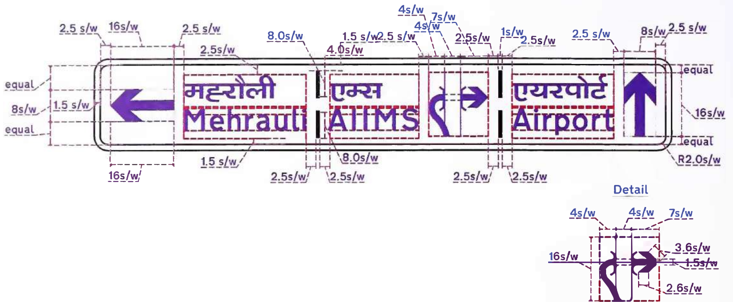
Fig. 16.16 Gantry Mounted Advance Direction Sign Ahead of a Flyover in Urban / City Roads
