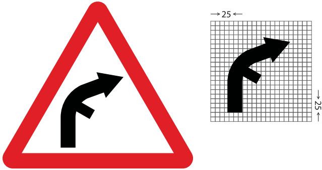
Fig 15.02a Right Side Road on Right Curve
