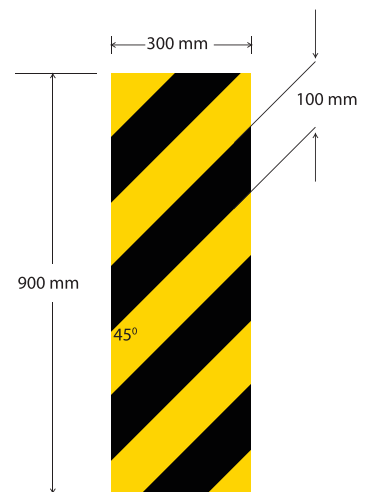
Fig 15.79 Object Hazard (Right)
