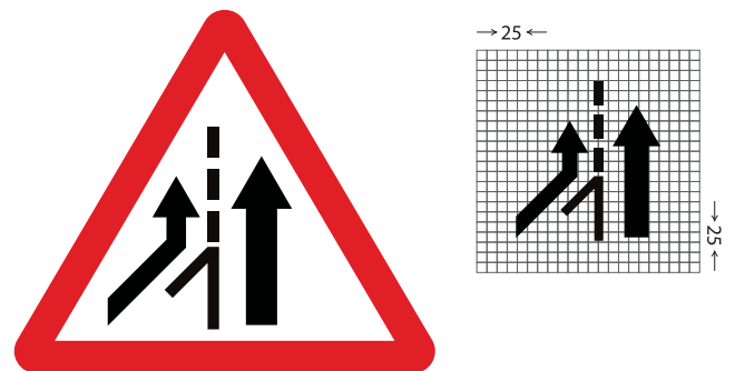
Fig 15.22 Merging Traffic Ahead (From Left)
