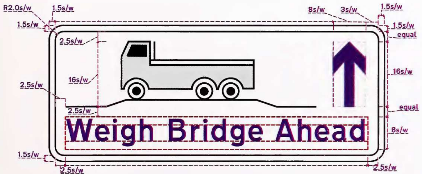
Fig. 16.09 Weigh Bridge Ahead
