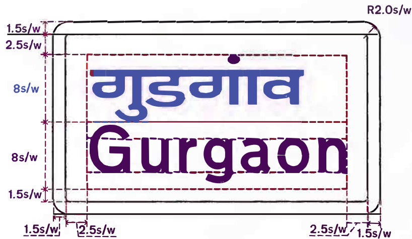
Fig. 16.06 Place Identification Sign
