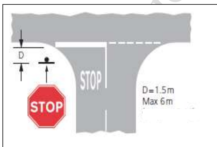
Figure 14.2: Location Description of STOP Sign
