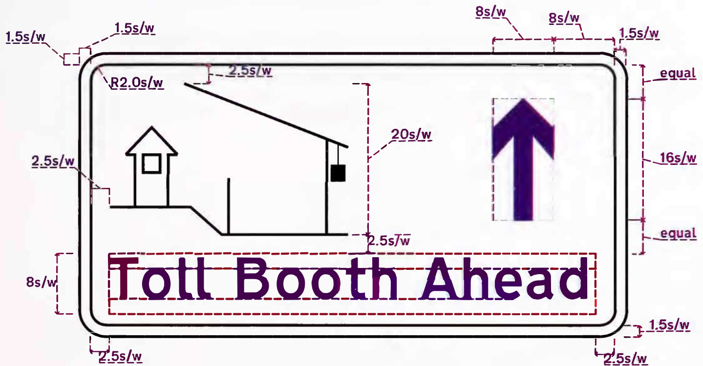
Fig. 16.08 Toll Booth Ahead
