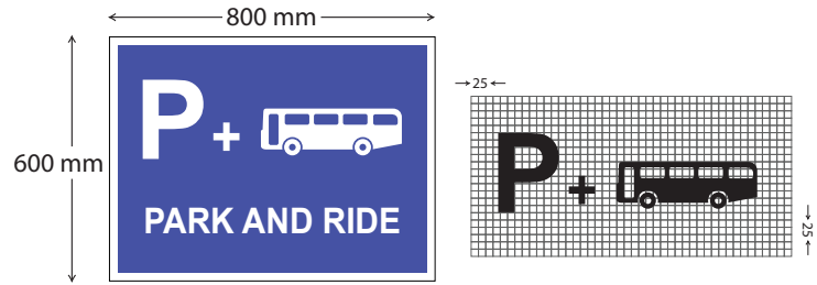
Fig 18.08 Park and Ride
