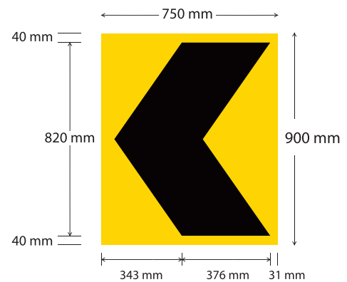
Fig 15.75 Single Chevron(>100kmph speed)
