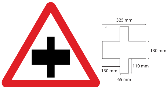
Fig 15.19 Major Road Ahead
