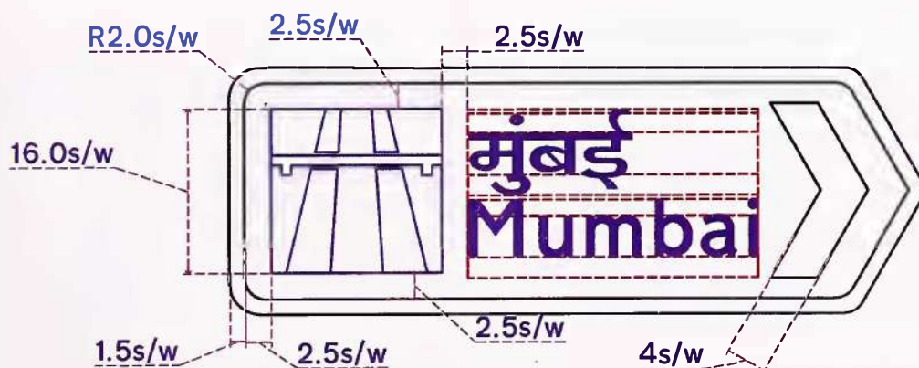
Fig. 16.15 Expressway Sign Ahead
