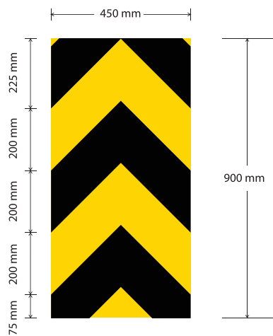
Fig 15.80 Object Hazard (Left)
