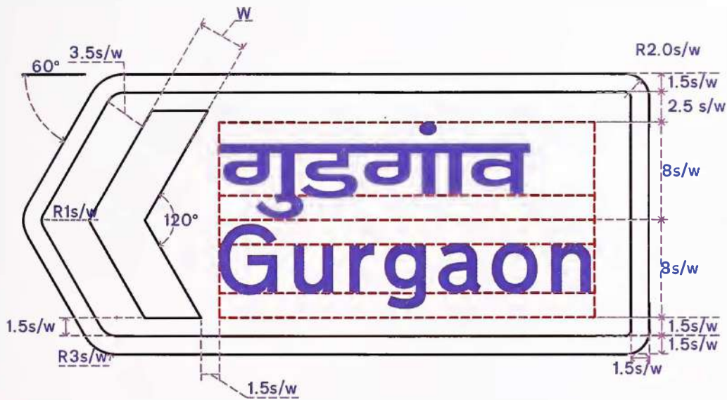
Fig. 16.04 Flag Type Direction Sign
