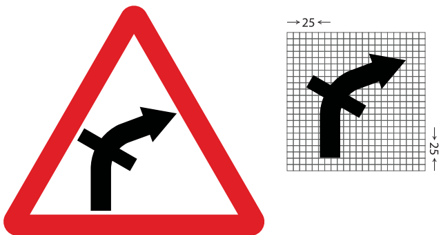
Fig 15.02c Cross Road on Right Curve
