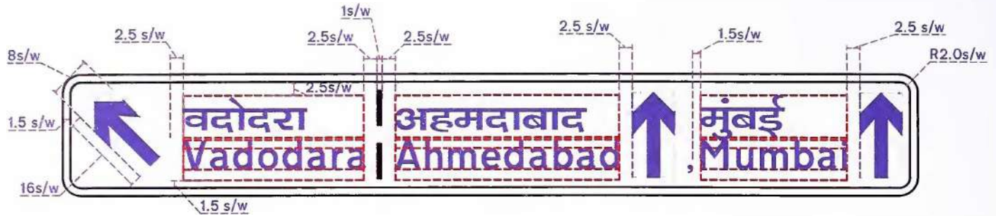
Fig. 16.10 Gantry Mounted Advance Direction Sign Ahead of a Grade Separated Junction
