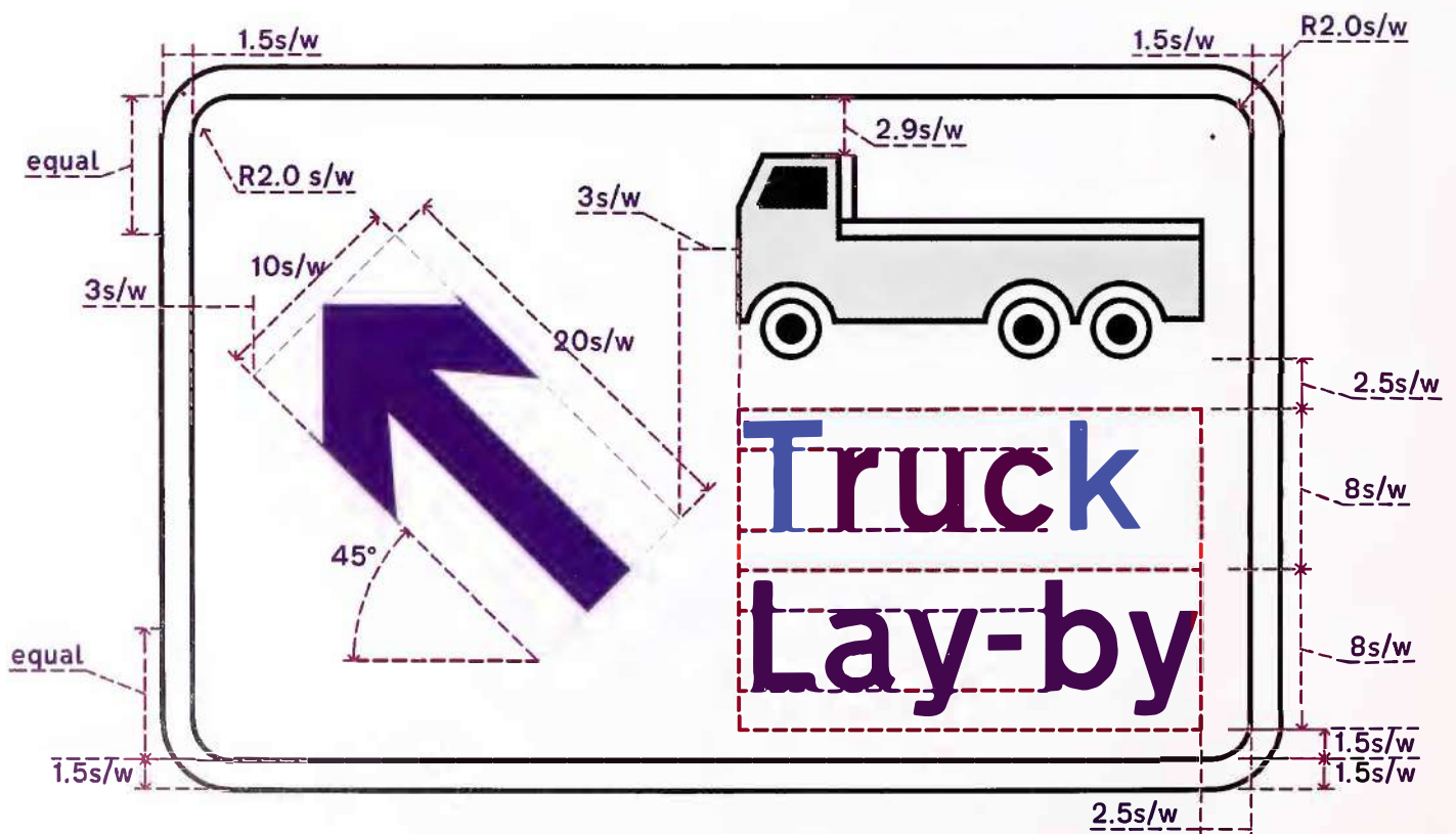
Fig. 16.07 Truck Lay- By
