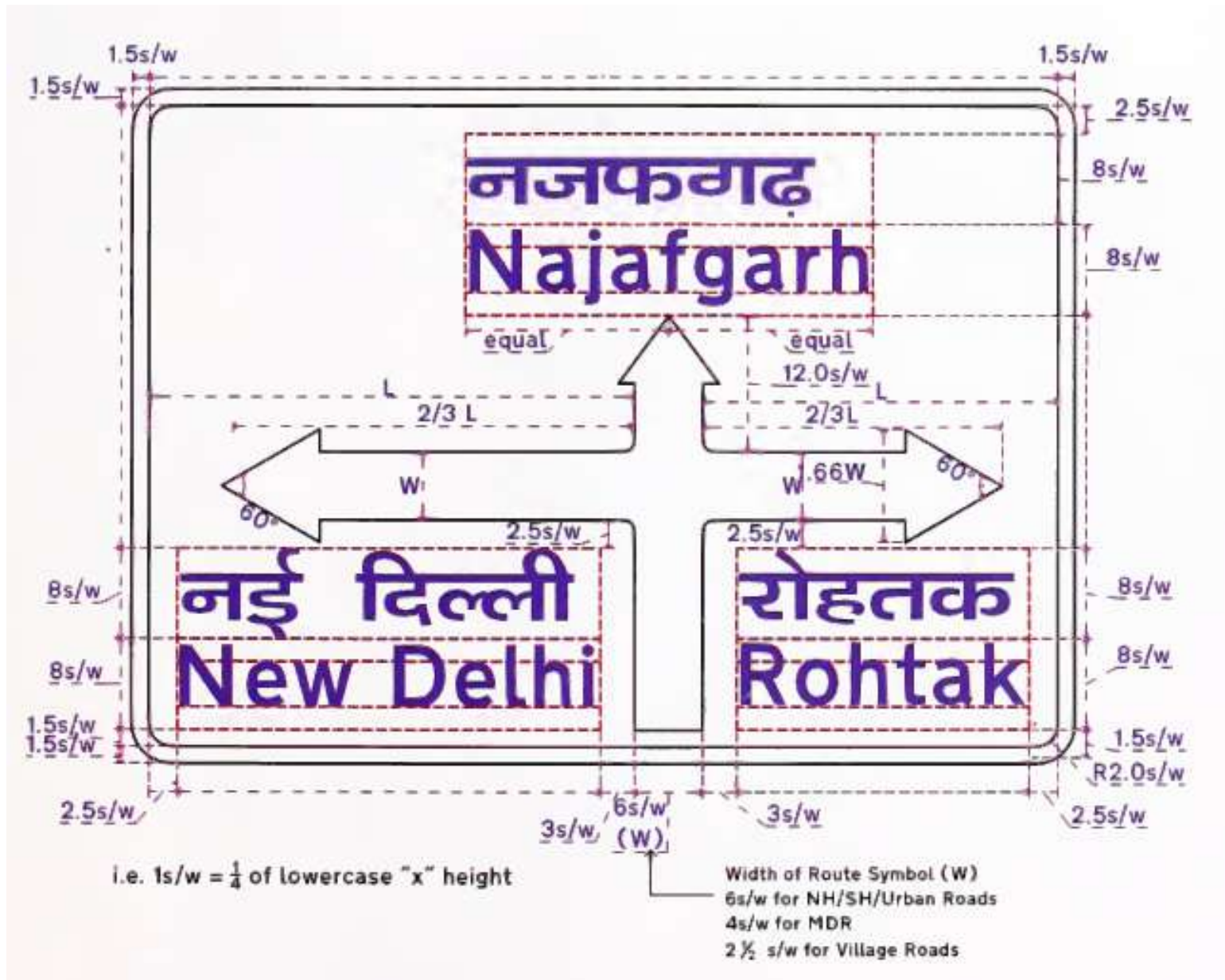
Fig. 16.02 Map type Advance Direction Sign (Shoulder Mounted)
