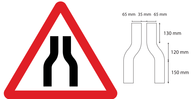
Fig 15.23 Narrow Road Ahead
