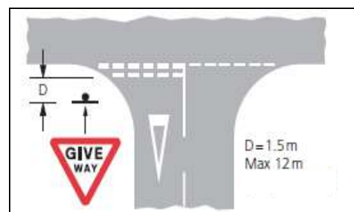
Figure 14.3: Location Description of GIVE WAY Sign
