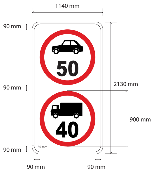
Fig 14.40 Maximum Speed Limit (Vehicle Type)
