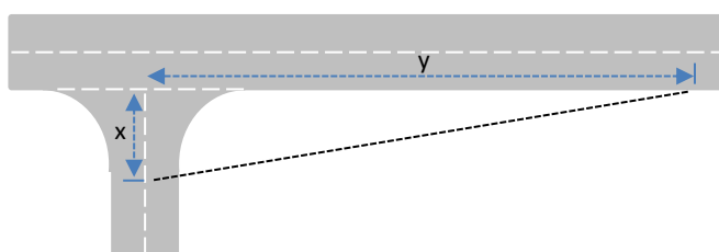
Figure 14.1: Description of Visibility Funnel
