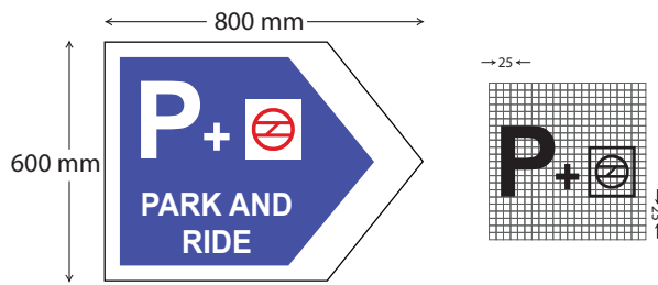
Fig 18.07 Park and Ride
