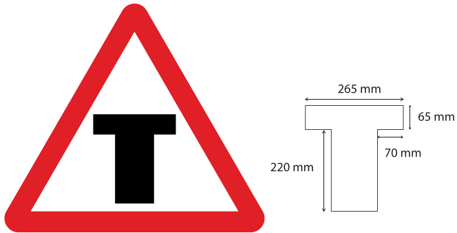
Fig 15.17 T-Intersection
