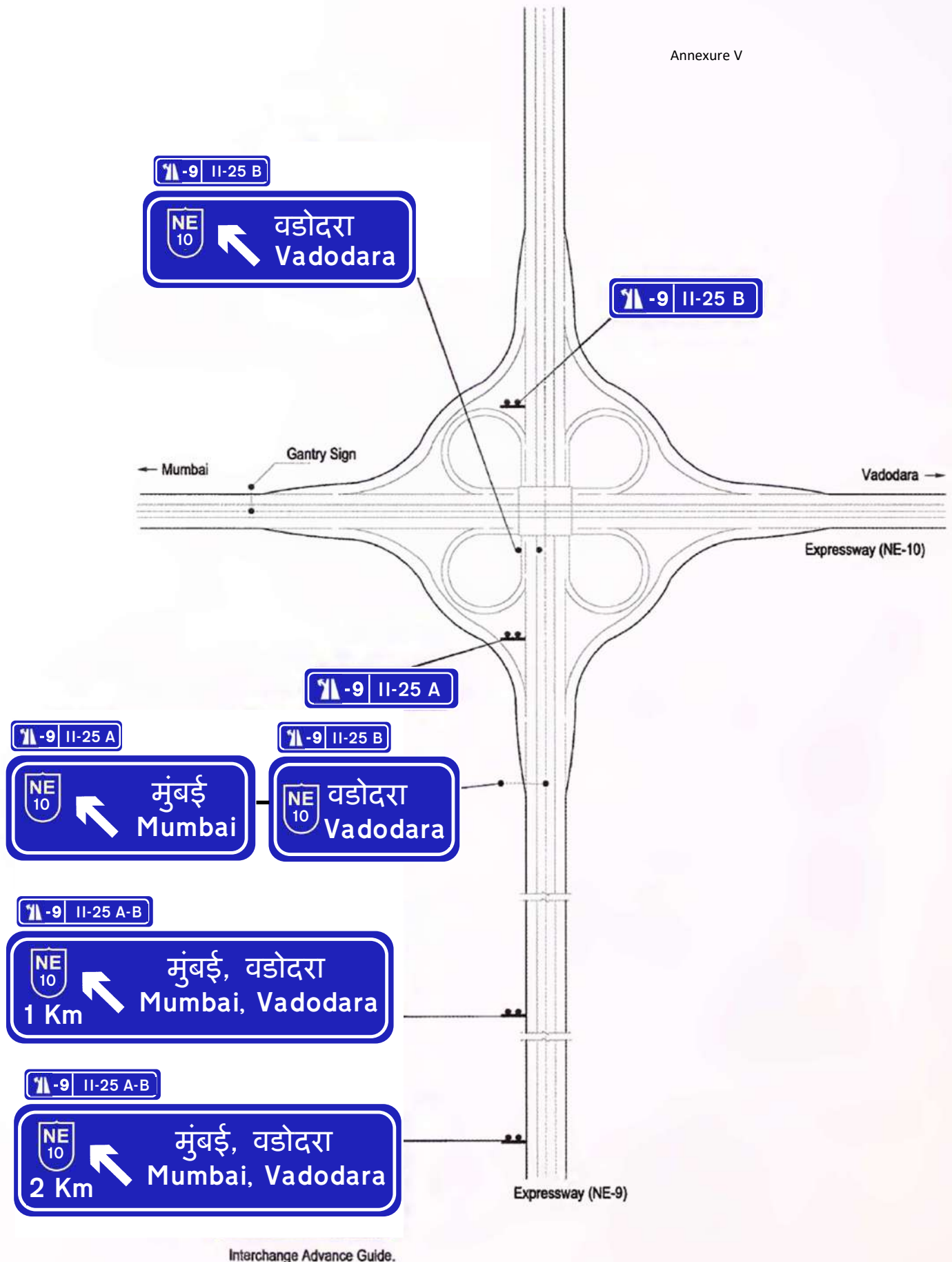
Fig. V.14: Typical Sign plan for Direction signs for Cloverleaf Interchange in an Expressway
