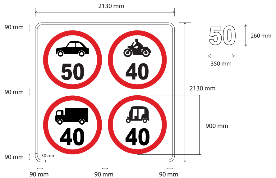
Fig 14.40a Maximum Speed Limit (Vehicle Type)
