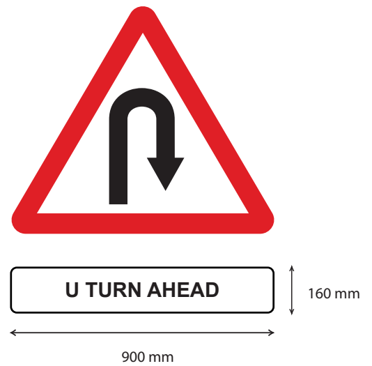
Fig 15.73 U Turn Ahead
