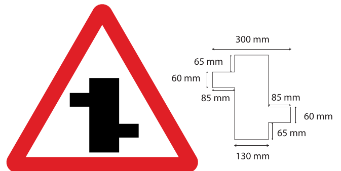
Fig 15.20 Staggered Intersection
