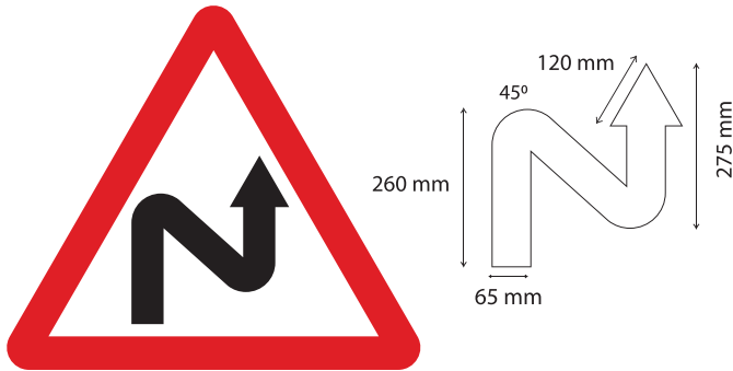
Fig 15.05 Right Reverse Bend
