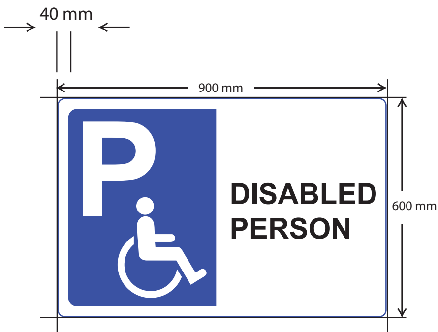
Fig. 19.02 Parking Information
