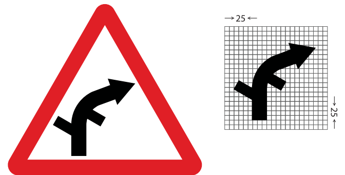
Fig 15.02d Staggered Intersection on Right Curve
