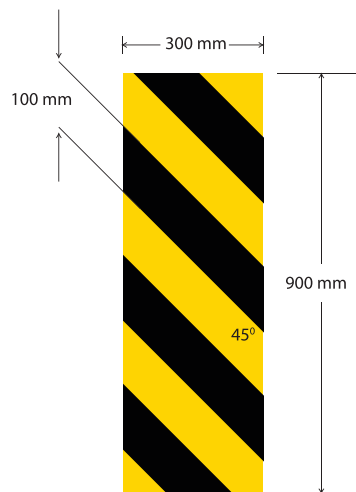
Fig 15.78 Object Hazard (Left)
