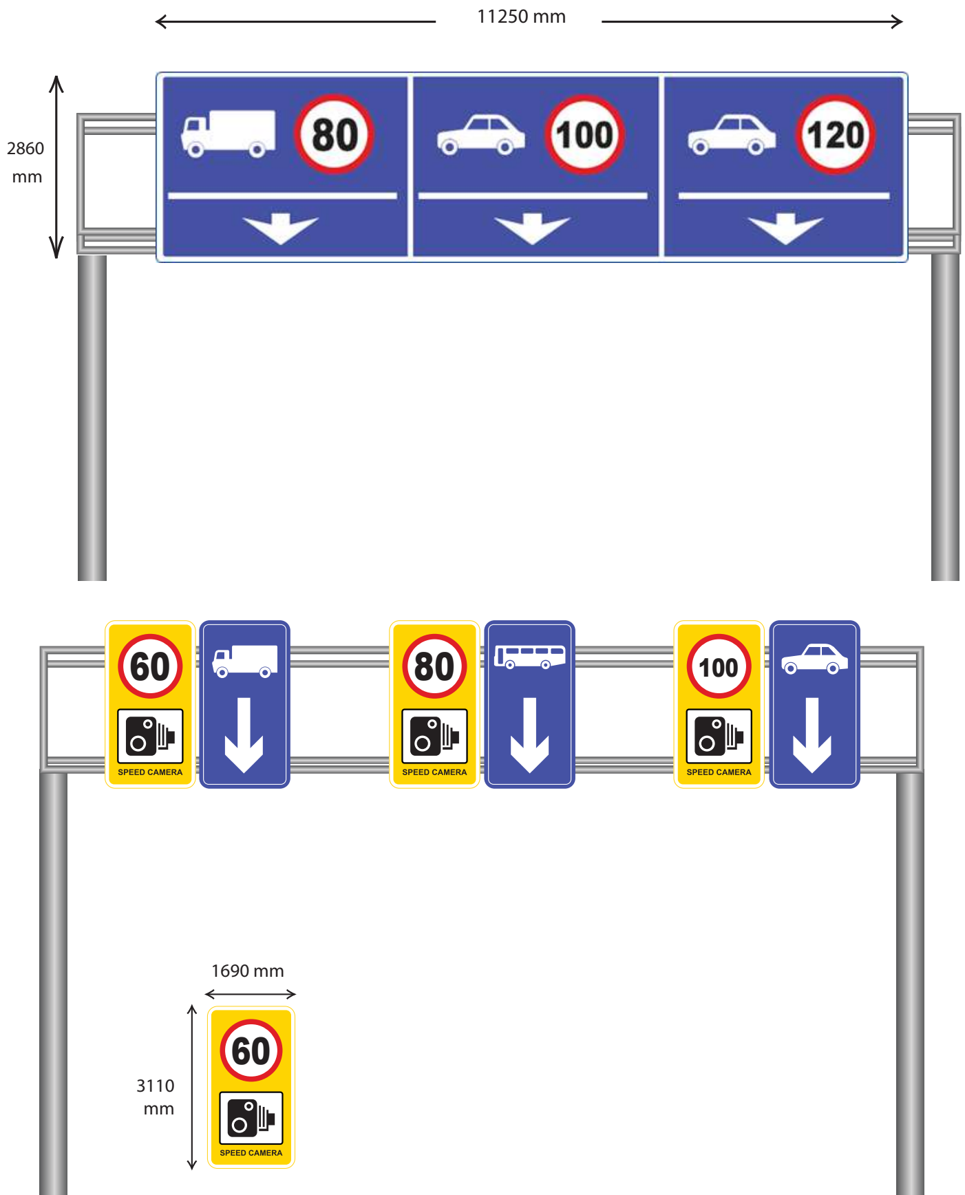
Fig 20.04 Vehicle Category wise and speed wise lane dedication information signs
