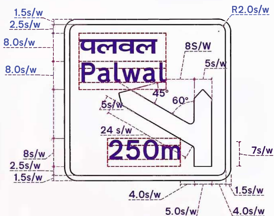
Fig. 16.14 Shoulder Mounted Sign in Advance of Grade Separated Junction
