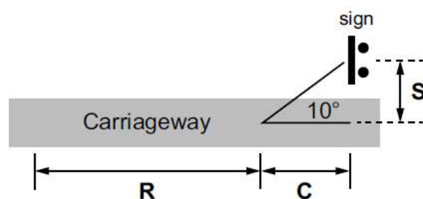
Figure VI.1: Description of Off-set, Cut-off and Reading Distances
