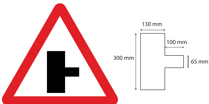
Fig 15.09 Side Road Right
