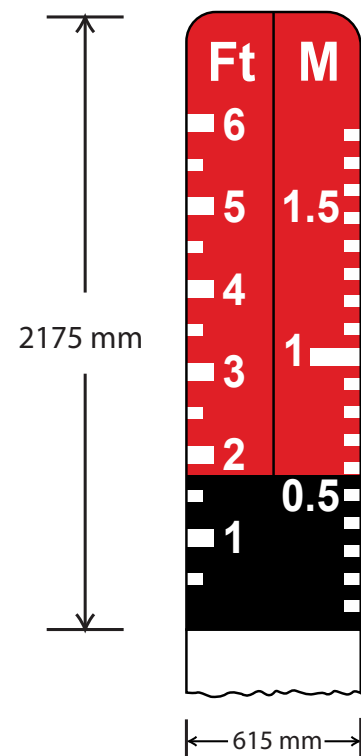
Fig 18.11 Flood Gauge
