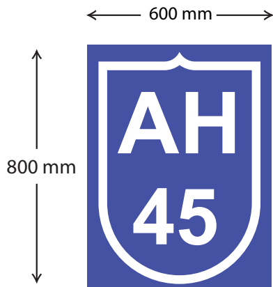
Fig 22.03 Asian Highway Route Marker Sign
