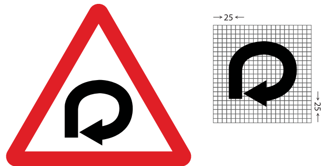
Fig 15.08 270 Degree Loop
